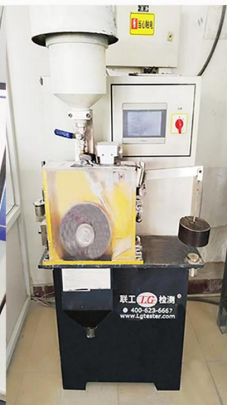
ASTM G65 Dry Sand Rubber Wheel Abrasion Tester
